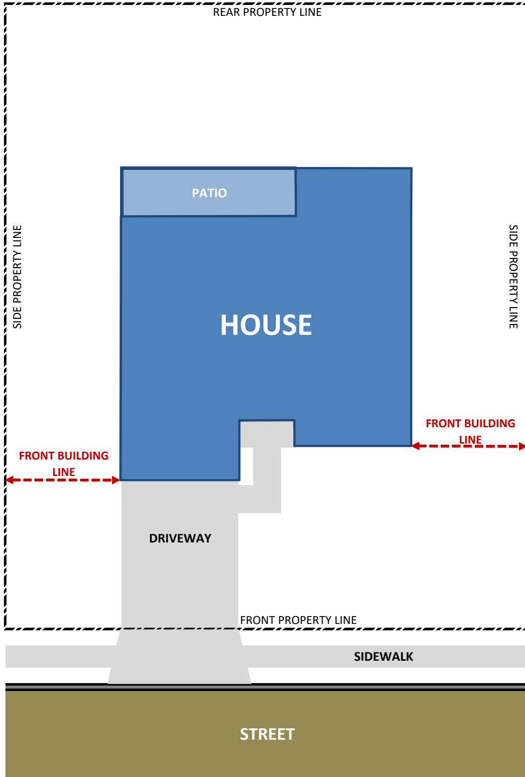
FIGURE 1 - INTERIOR LOT
